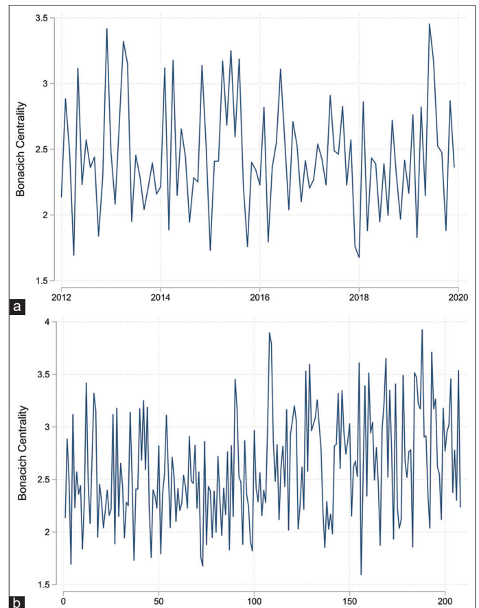
Figure 10: \mu for water inflows of plants. (a) Monthly. (b) Biweekly
