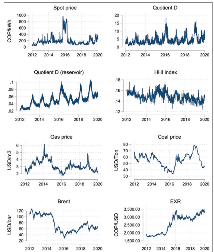
Figure 6: Spot price and fundamental variables
