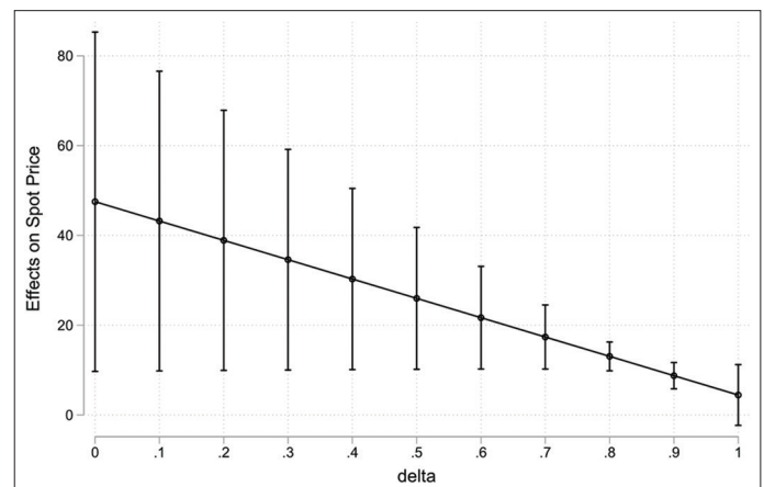
Figure 7: Average marginal effects of demand/water inflows (MoE) with 95% Cis
