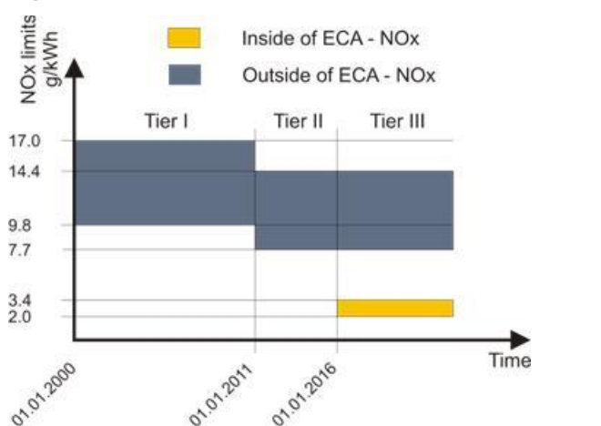
Fig. 2 Emission limit for NOx (IMO, Annex VI, the regulation 13)
