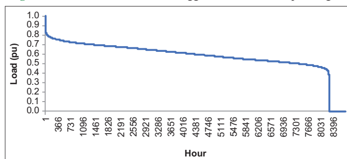
Figure 6: LDC of Sulawesi Nusatenggara and Maluku Papua Region
