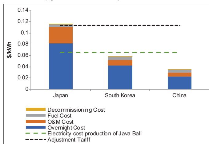
Figure 8: Comparison of NPP's LUEC on each country to the electricity production cost and adjustment tariff in Java Bali
