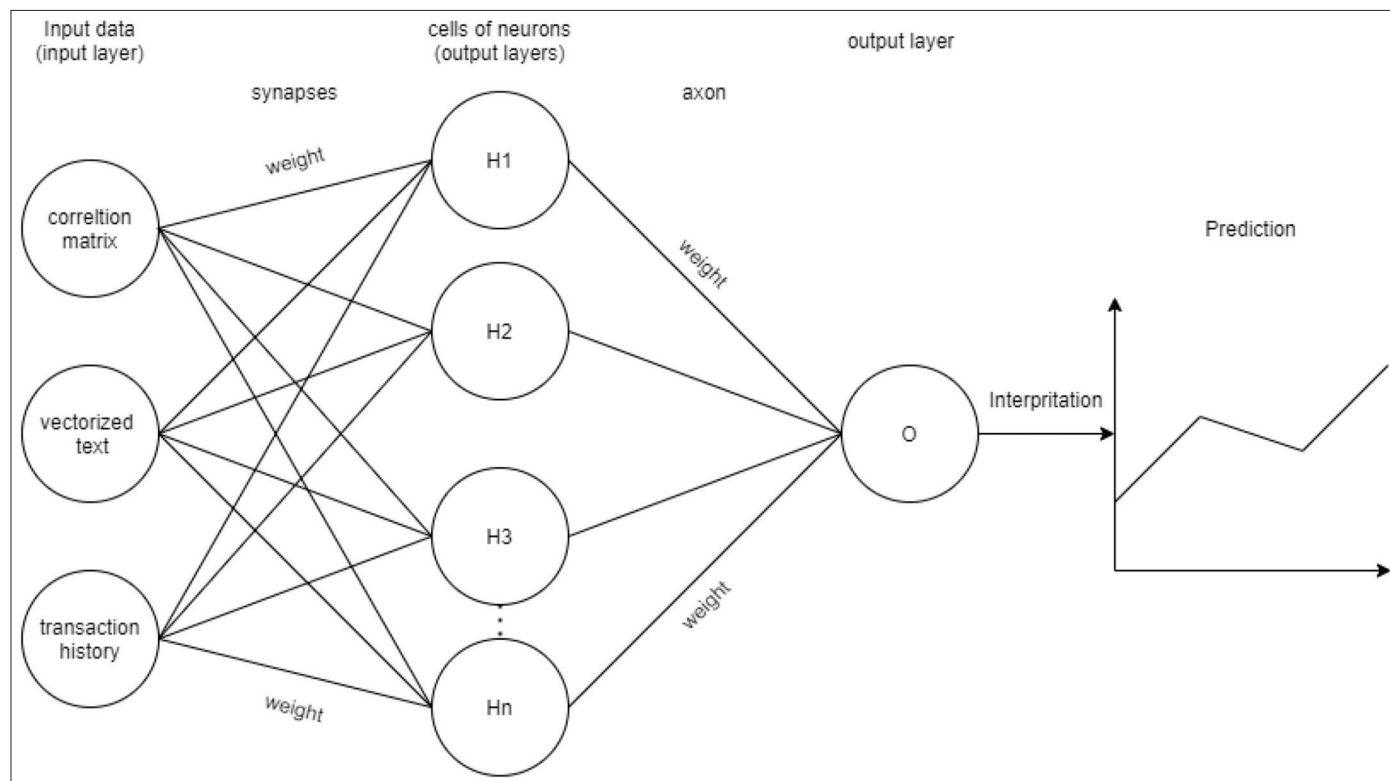
Figure 3: Diagram of an artificial neural network
