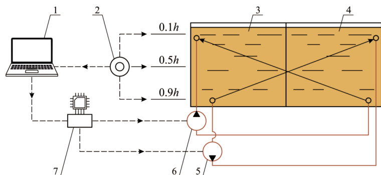
Fig. 2. Providing additional circulation of the drilling slurry in the cargo tanks of the vessel and the technology for carrying out experimental work: 1 – laptop; 2 – hydrometer; 3, 4 – cargo tanks for transportation of drilling slurry; 5, 6 – additional circulation pumps; 7 – microcontroller
