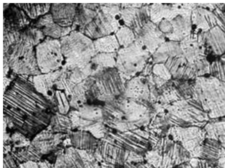
Fig. 1. The microstructure of steel 110G13 in the cast state (×500)
