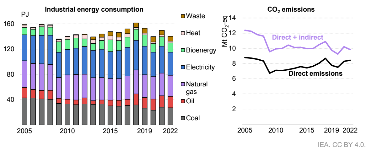
Figure 2.4 Energy demand and emissions from industry in the Slovak Republic, 2005-2022
