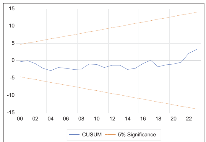
Figure 2: CUSUM test
