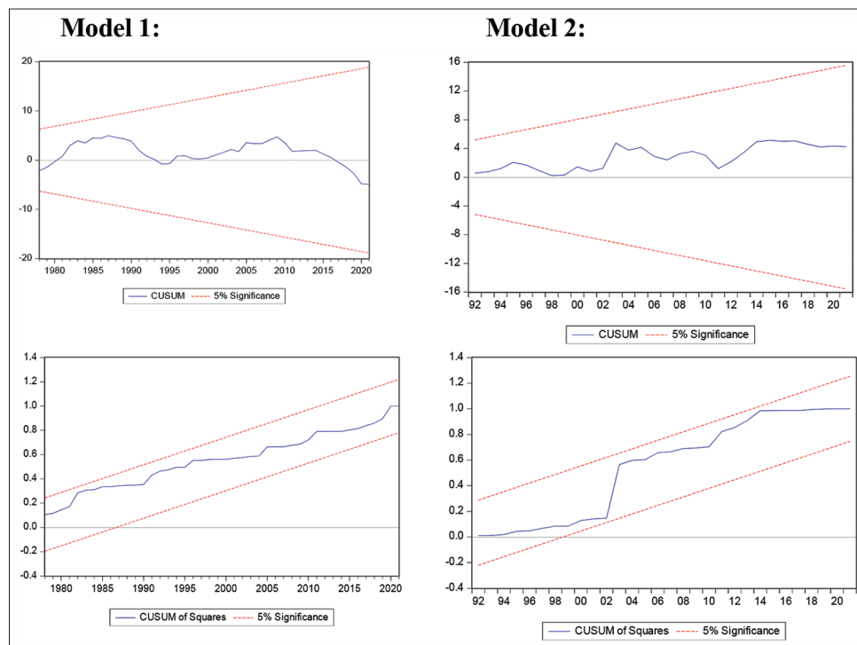
Figure 1: CUSUM graphs
