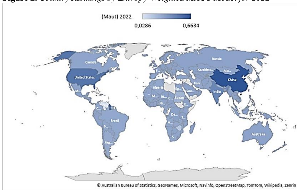
Figure 2. Country Rankings by Entropy-Weighted MAUT Model for 2022
