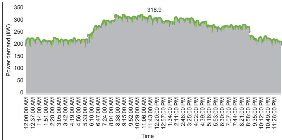
Figure 3: Load profile at the PCC
