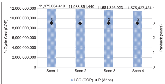
Figure 6: Life cycle cost and payback period for each scenario. Where P is the payback period
