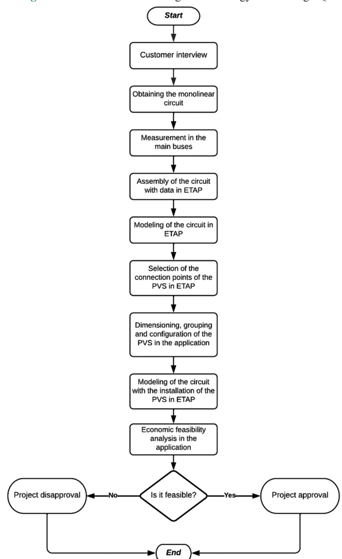
Figure 1: Flowchart of PVS design methodology considering PQ
