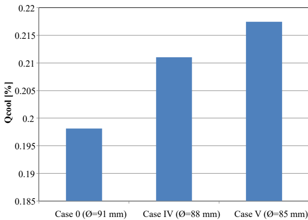
Fig. 10. Heat ratio in the exhaust
