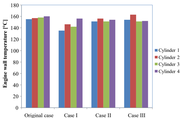
Fig. 7. Wall temperature of the different cylinders
