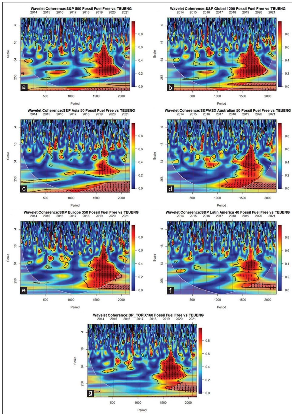
Figure 3: (a-g) S&P Fuel free indices and twitter economic uncertainty. Presents the results of wavelet coherence between returns of S&P fossil-fuel-free indices and Twitter economic uncertainty which is the second series. The color heat map displays the intensity of co-movement which ranges from blue (close to zero) to red to high (close to one). The direction of co-movement between two-time series x and y in the wavelet coherence plot is explained with arrows. Where, rightward-directed arrows \rightarrow : “x” and “y” show in-phase (Positive co-movement), leftward-directed arrows \leftarrow : “x” and “y” indicate an anti-phase relationship (Negative co-movement).” While downward arrows indicate \downarrow : “x” leading “y” by “90° (First Series is Leading) and \uparrow : “y” leading “x” by “90° (Second Series is Leading). Source: Datastream database
