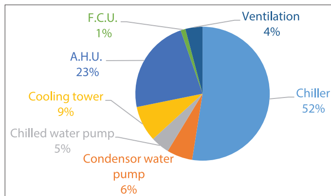
Figure 2: This is energy consumption percentage of air conditioning system by each machine of building study case
