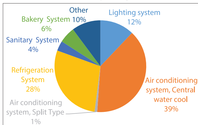
Figure 1: This is an energy consumption percentage by each system of case study building
