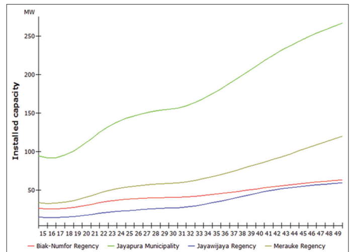
Figure 6: Installed capacity increases of the power plants in the BaU scenario
