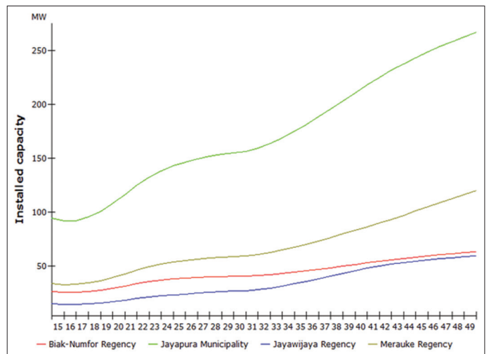
Figure 6: Installed capacity increases of the power plants in the BaU scenario
