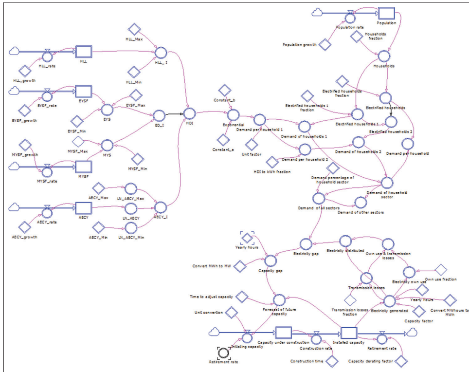
Figure 3: System dynamics model of electrical systems in Papua Province
