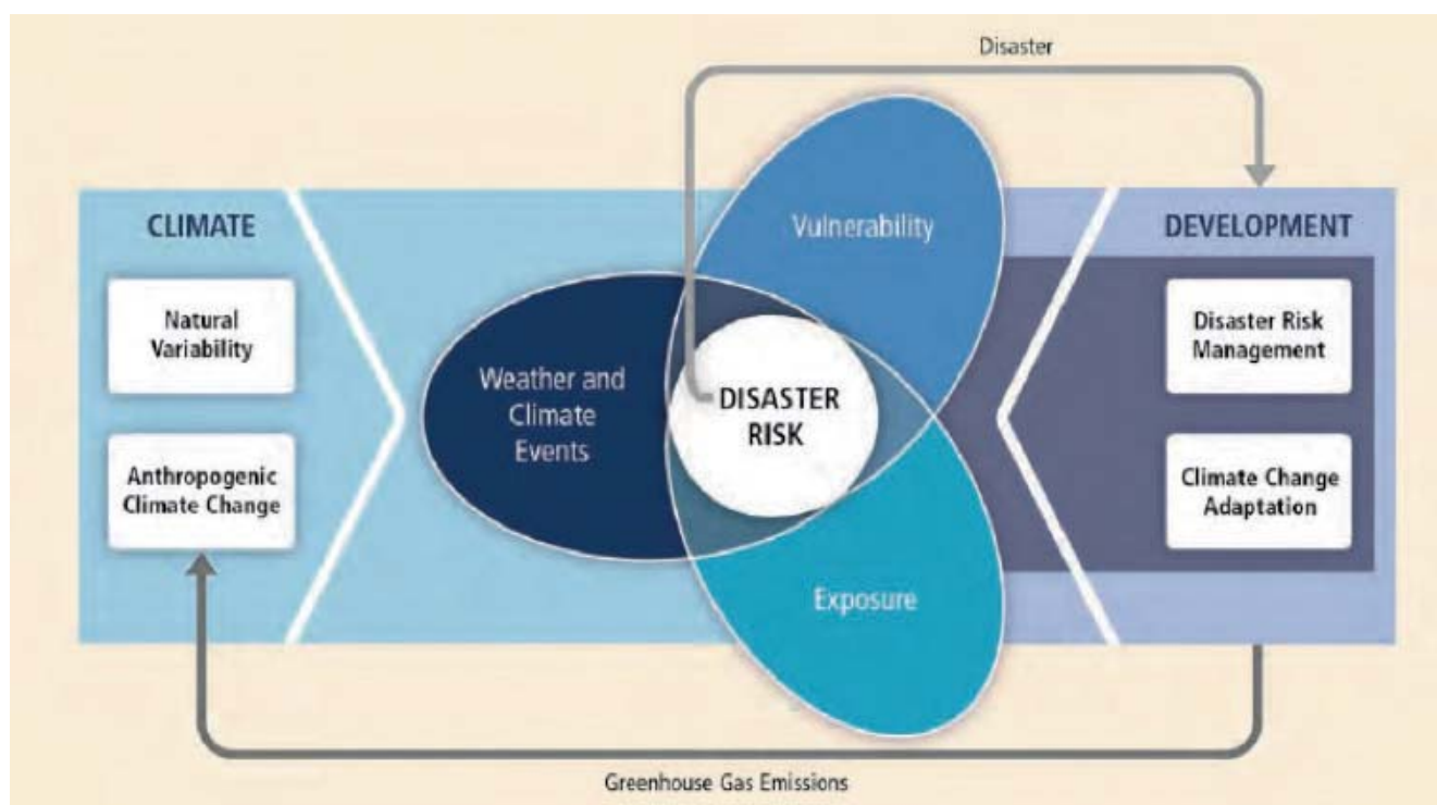
Figure 1.11 Climate extremes, exposure and vulnerability
