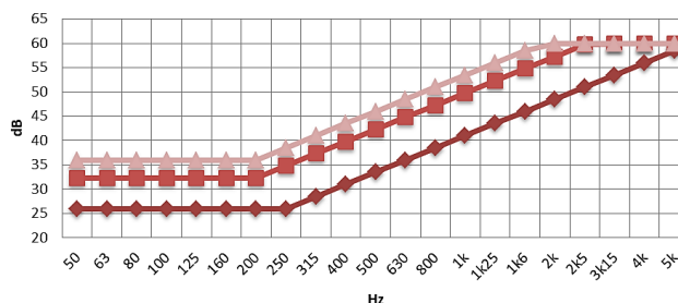
Fig. 4. Sound insulation frequency response for aerated concrete walls with density 800 kg/m 3 and different thicknesses: — 100 mm; — 200 mm; — 300 mm
