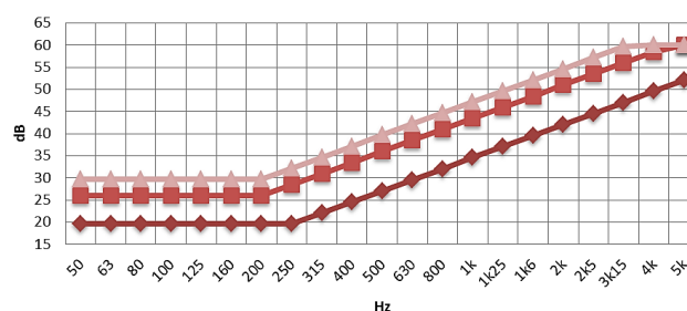
Fig. 2. Sound insulation frequency response for aerated concrete walls with density 400 kg/m 3 and different thicknesses: — 100 mm; — 200 mm; — 300 mm
