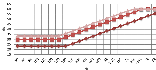
Fig. 3. Sound insulation frequency response for aerated concrete walls with density 600 kg/m 3 and different thicknesses: — 100 mm; — 200 mm; — 300 mm
