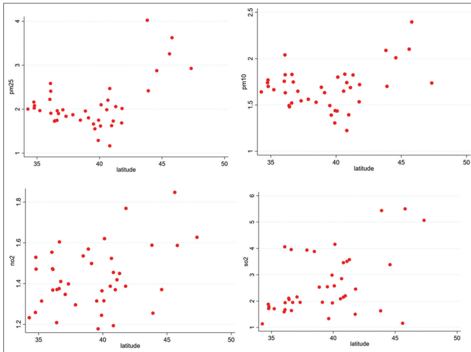
Figure 3: Scatter diagrams between heating ratios and latitudes (2015-2019)
