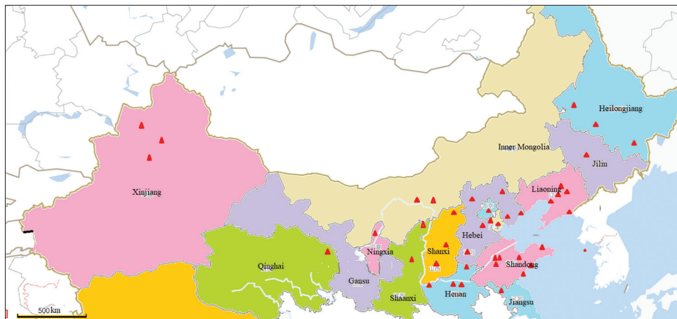
Figure 1: Heating cities in North China
