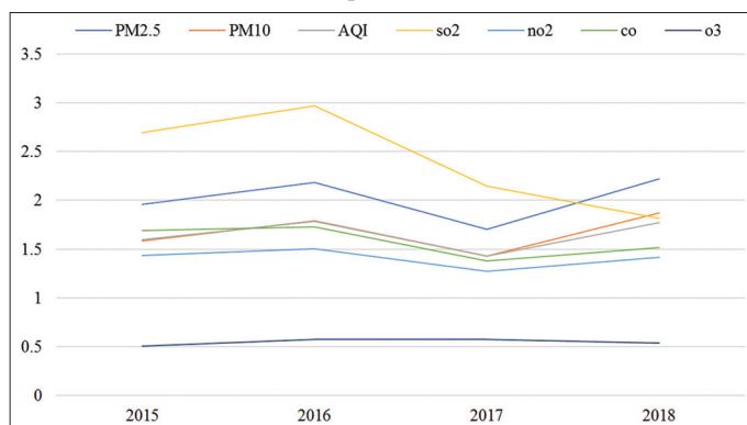
Figure 4: Time series for average heating ratios in terms of different air pollutants
