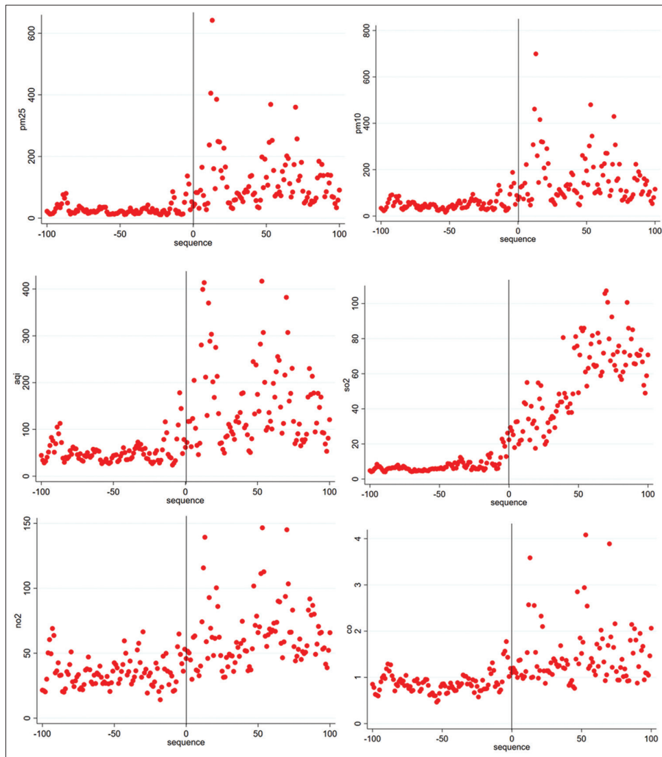
Figure 6: Plot of average pollutants' level and days using real data, PM2.5, PM10, AQI, SO2, NO2, CO respectively
