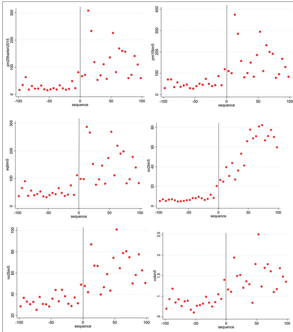
Figure 5: Plot of average pollutants' level and days using bin size 5 data, PM2.5, PM10, AQI, SO2, NO2, CO respectively
