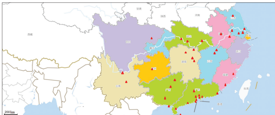
Figure 2: Non-heating cities in South China
