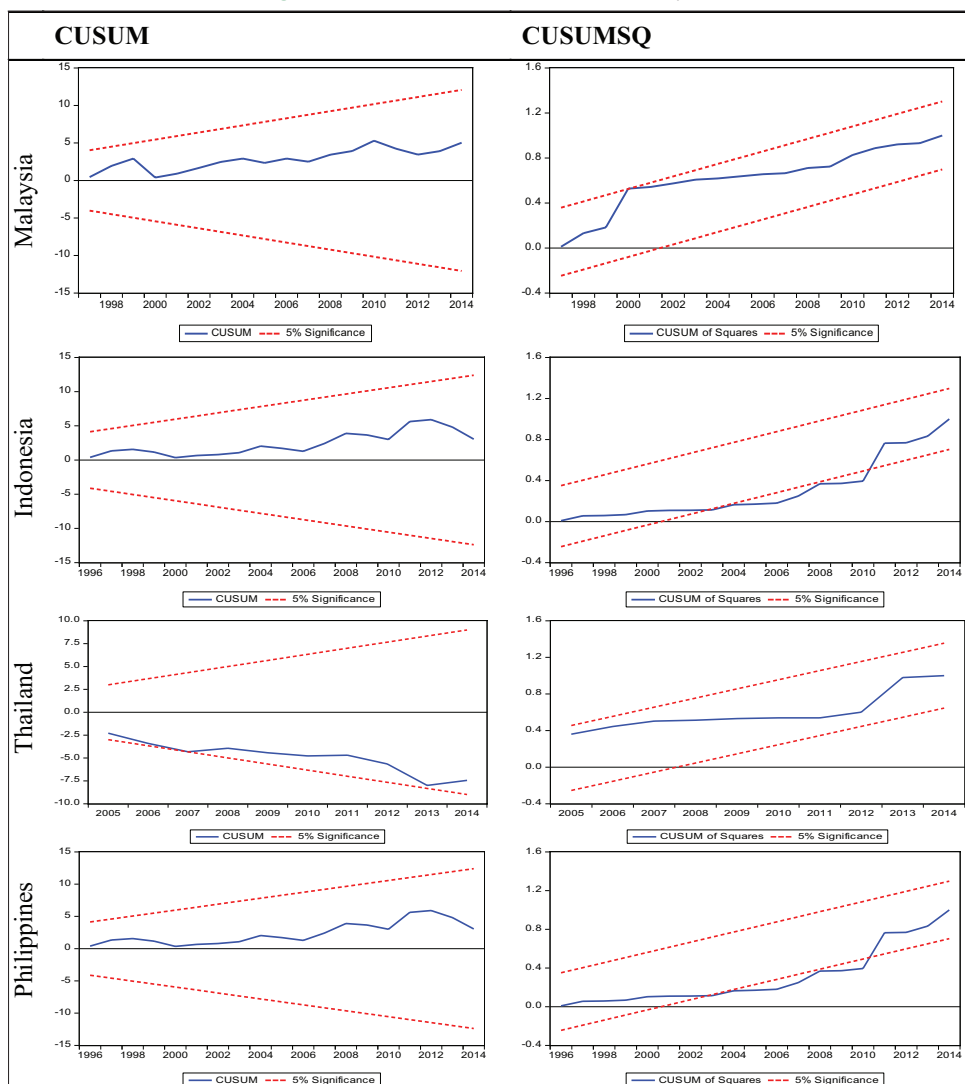
Figure 3: CUSUM and CUSUMSQ stability test
