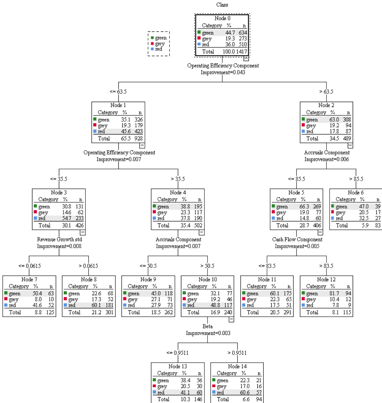
Figure 2: CRT regression tree representation (Source: authors' projection with SPSS 19.0)
