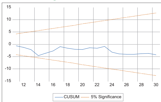
Figure 2: CUSUM Zimbabwe
