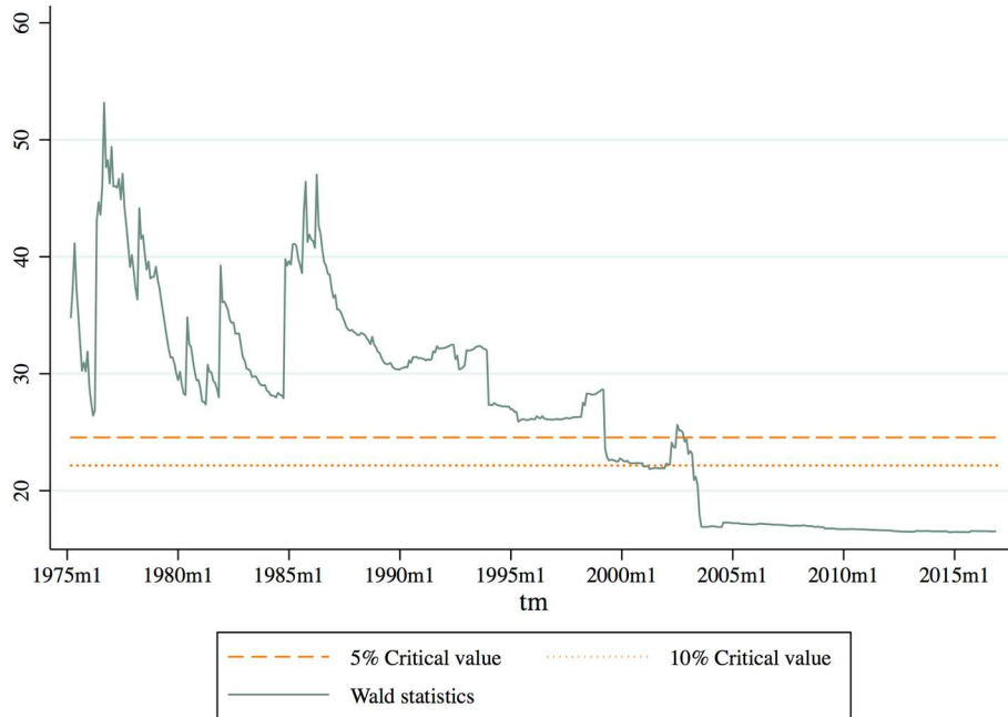
Figure 2: Wald statistics testing whether inflation ( \pi_t ) Granges-causes inflation uncertainty ( h_t ) against the alternative of a break in Granger causality at time tm (reported on x-axis)
