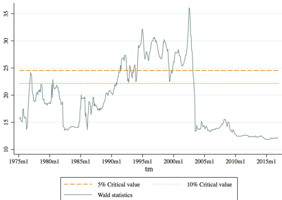
Figure 3: Wald statistics testing whether inflation uncertainty ( h_t ) Granges-causes inflation ( \pi_t ) against the alternative of a break in Granger causality at time tm (reported on x-axis)
